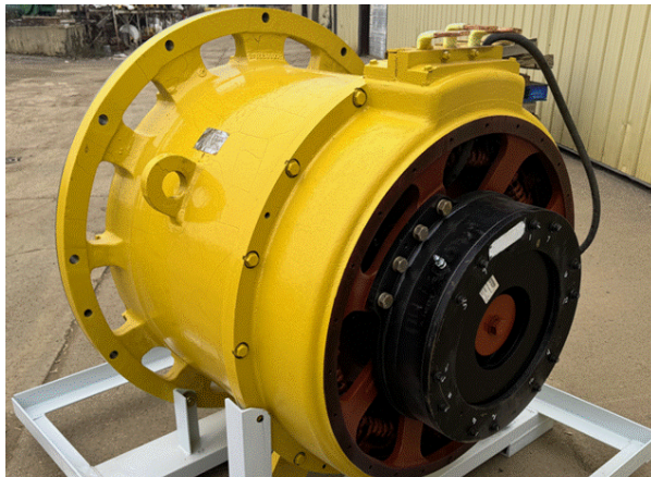
5GEB16 | Traction Motor (With Optional Brake)
